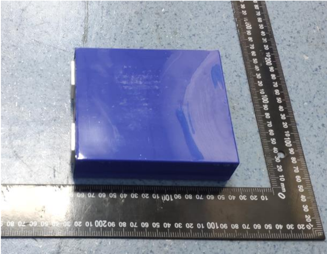
Cells /电芯 (36130145 3.2V 52.5Ah 168Wh)
